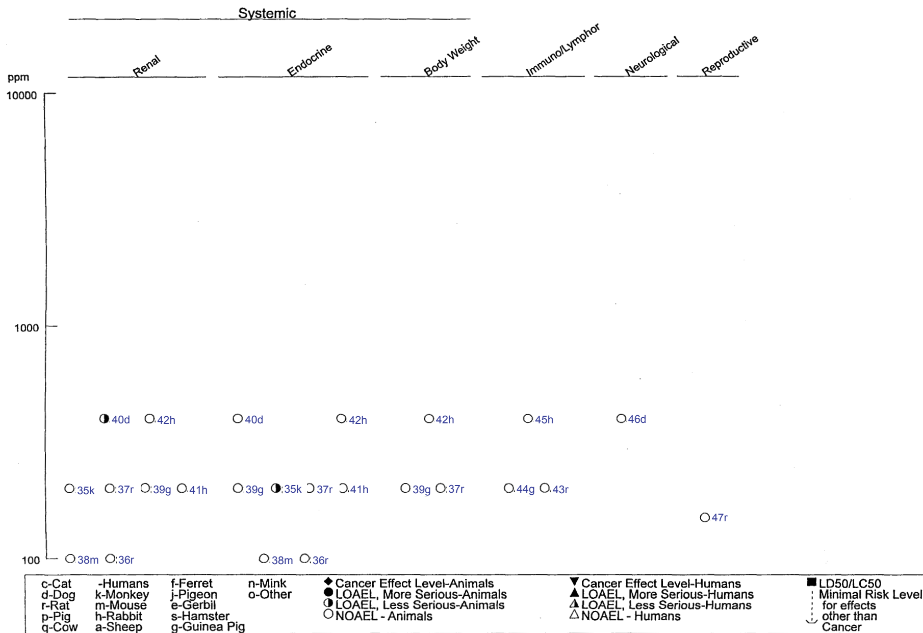
Figure 3-1. Levels of Significant Exposure to 1,2-Dichloroethane - Inhalation (continued) Intermediate (15-364 days)
